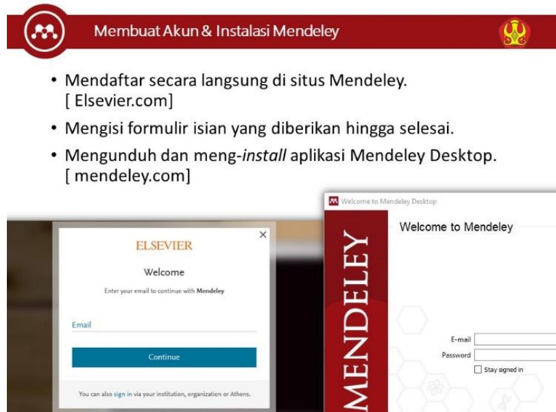
Gambar 3 Penginstalan Mendeley
